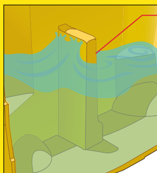
Molded-in wave brake
